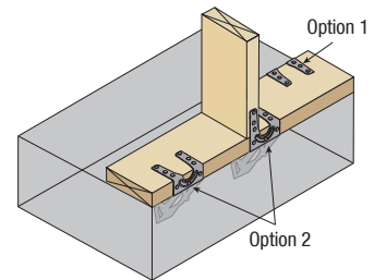
Field bend and attach
