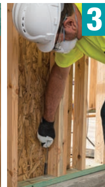
3 Blow out hole with compressed air; brush; blow again
