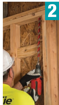
2 Drill top hole through the plate
