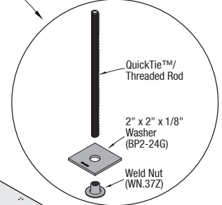
Weld Nut for QuickTie™/ Threaded Rod to Lintel Attachment
