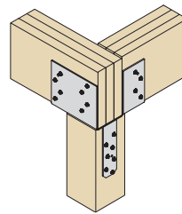
ECCSLL (End Column Cap w/ Left Leg Beam) (Part includes structural wood screws)
