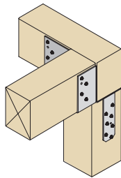
ECCSLR (End Column Cap w/ Right Leg Beam) (Part includes structural wood screws)
