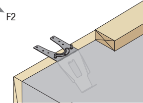
Option 2: Placement for outside wall attachment
