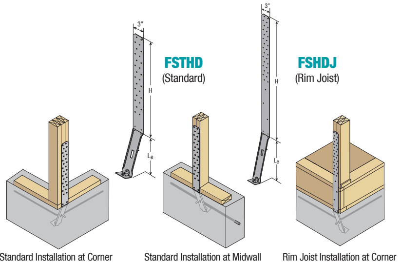
Standard Installation at Corner
