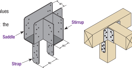
CCST (Column Cap w/ Tee Beam) (Part includes structural wood screws)
