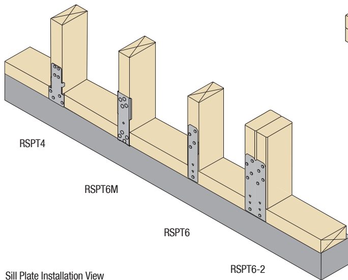
Sill Plate Installation View
