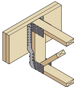
Face Mount
