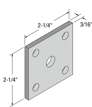
BPBC2.25-33N (QTB) BPBC2.25-33NS (QTB)
