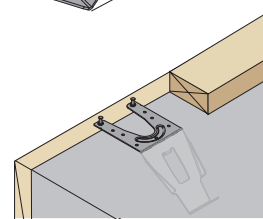
Option 1: Placement for inside wall attachment
