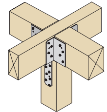
CCSC (Column Cap w/ Cross Beams) (Part includes structural wood screws)
