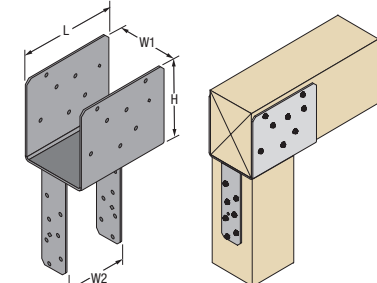
ECCS (End Column Cap) (Part includes structural wood screws)
