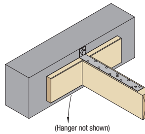
LTT20 as Tension Tie
