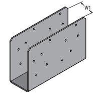
CCSO (Column Cap w/ No Straps) (Part includes structural wood screws)
