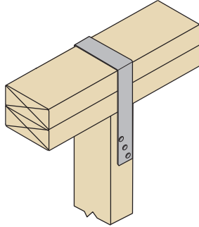
SPT Series to Bottom Plate and Top Plates
