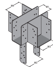
CCSC (Column Cap w/ Cross Beams) (Part includes structural wood screws)
