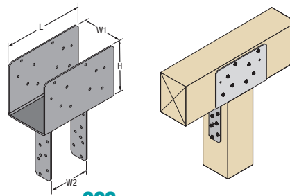
CCS (Column Cap) (Part includes structural wood screws)
